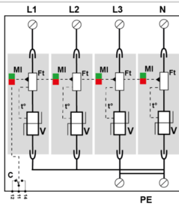
V: High-energy varistor Ft: Thermal fuse C: Remote signal contact t°: Thermal disconnection system MI: Disconnection indicator
